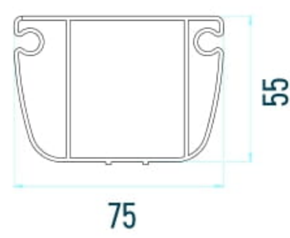
DOUBLE FABRIC PROFILE
